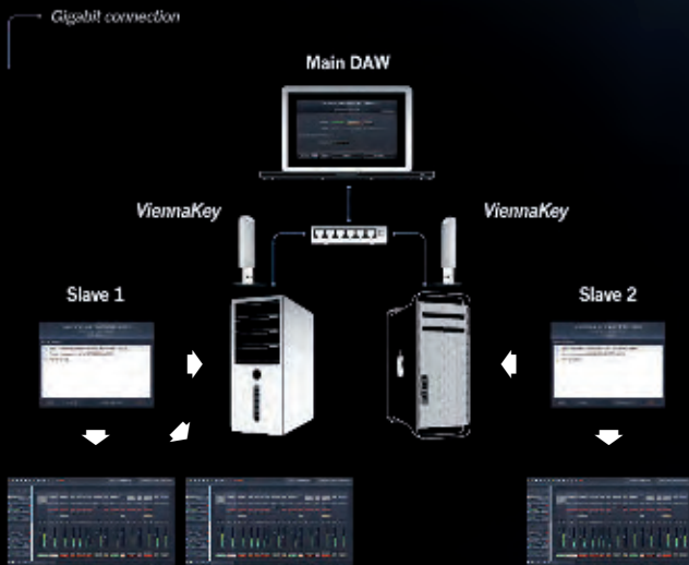
LAN Setup with three Computers
